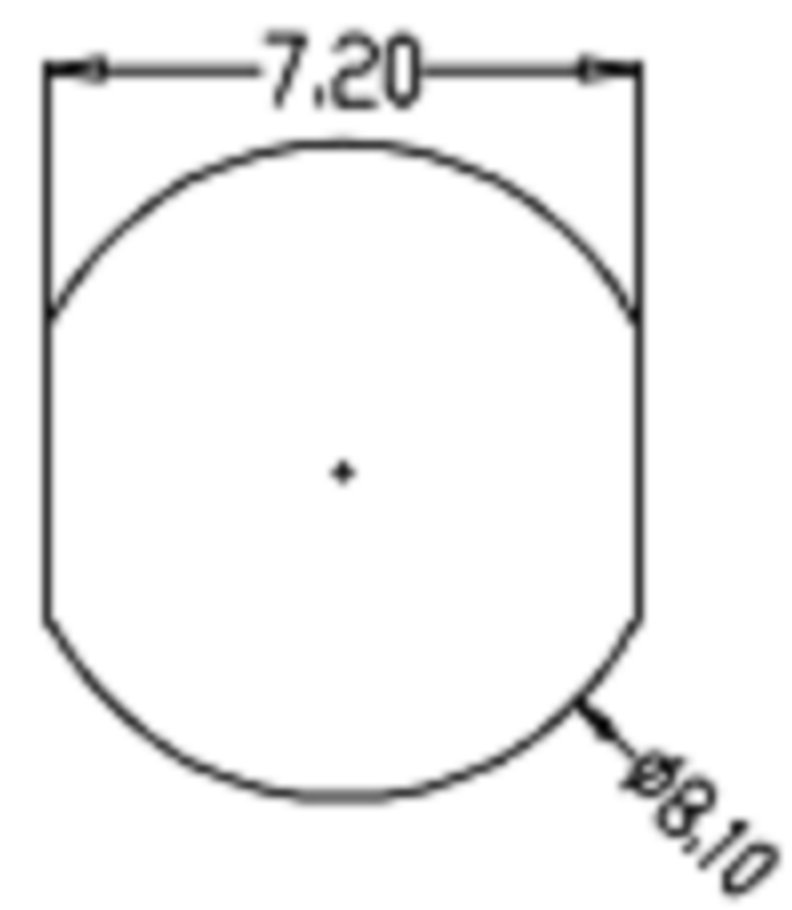
Recommended Panel Cut-out
