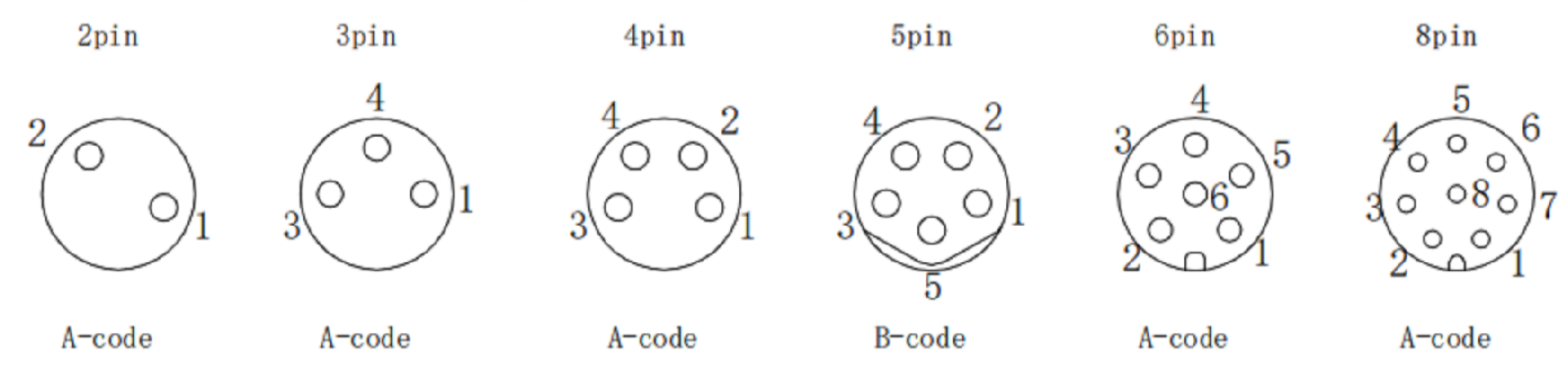
Pin assignment front view/针位分布前视图
